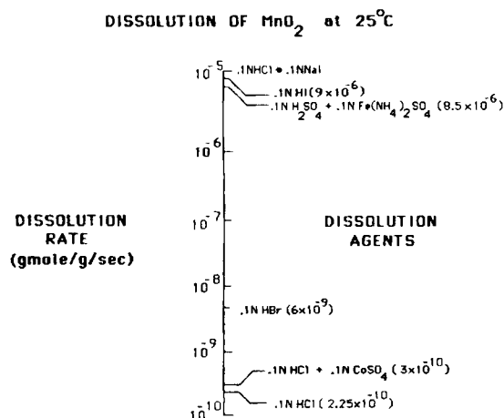
Figure 11. Effect of \text{Fe} and \text{Co} couples on \text{MnO}_2 dissolution.
