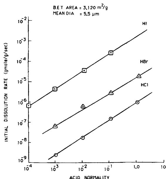
Figure 5. Dissolution of \text{Mn}_3\text{O}_4 in halogen acids at 25°C.
