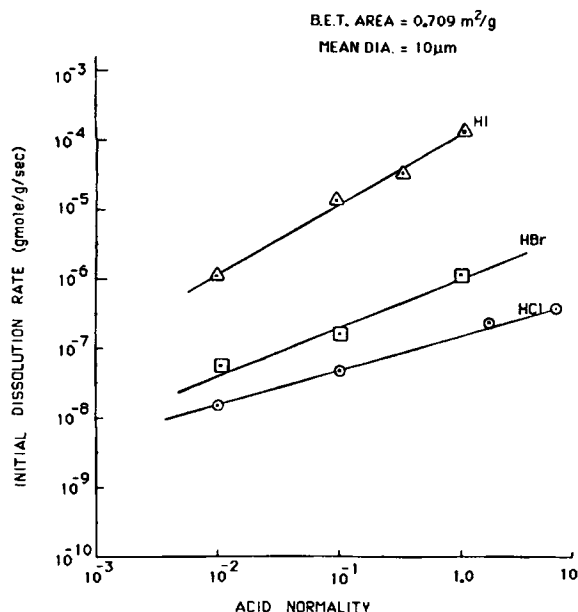
Figure 4. Dissolution of \text{Mn}_2\text{O}_3 in halogen acids at 25°C.
